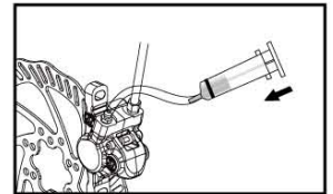
f-4. Fill the reservoir with oil by pushing the syringe
