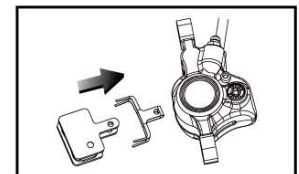
e-2. Replace pads and holder
