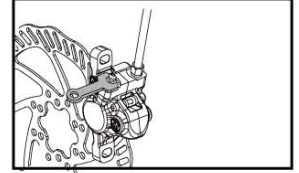
f-3. Open the outlet valve 1/4 turn
